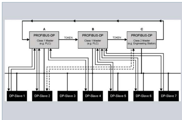
Figure 7: Profibus scan
