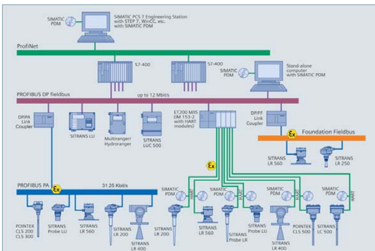
Figure 6: Profibus network
