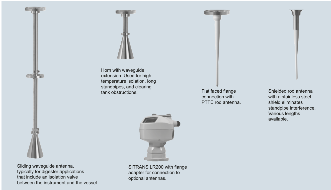
Antenna configurations for SITRANS LR200
