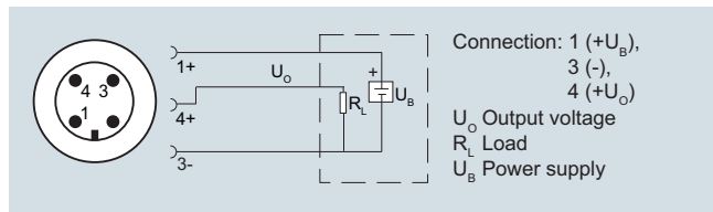
Connection with voltage output, ratiometric output and M12x1 plug
