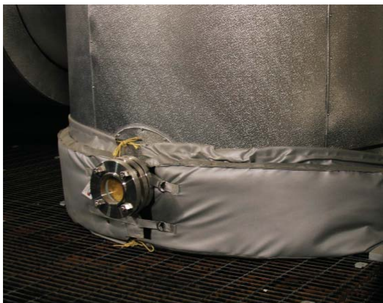
Kawartha Ethanol uses extra wraps of removable, customized insulation to reduce heat loss in crucial areas.
