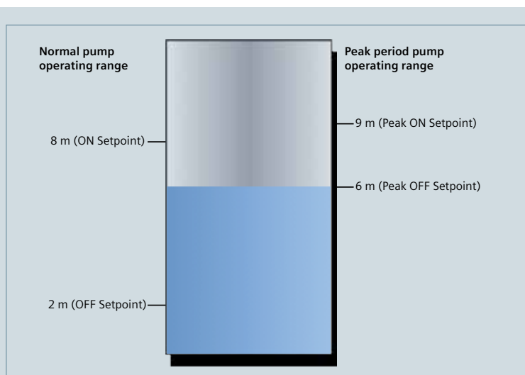
Figure 1: During peak periods, the pump operating range is much smaller than in normal operation, reducing the amount of time pumps must run.
