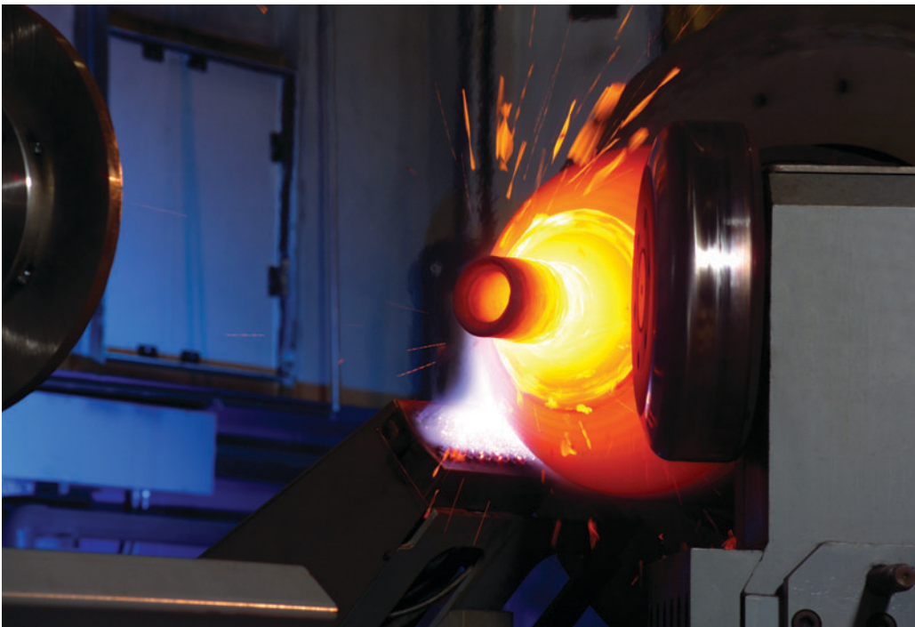
An induction heating system and shaping tools close the end of the steel tube for seamless integrity, a substantial improvement over welded end caps
