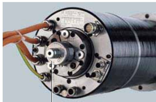
Rotary unit for internal tool cooling
